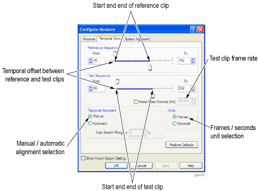
Figure 2: Temporal Sync tab
